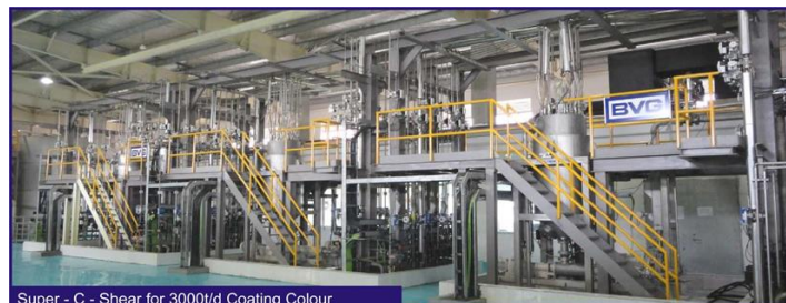
Super - C - Shear for 3000l/d Coating Colour
